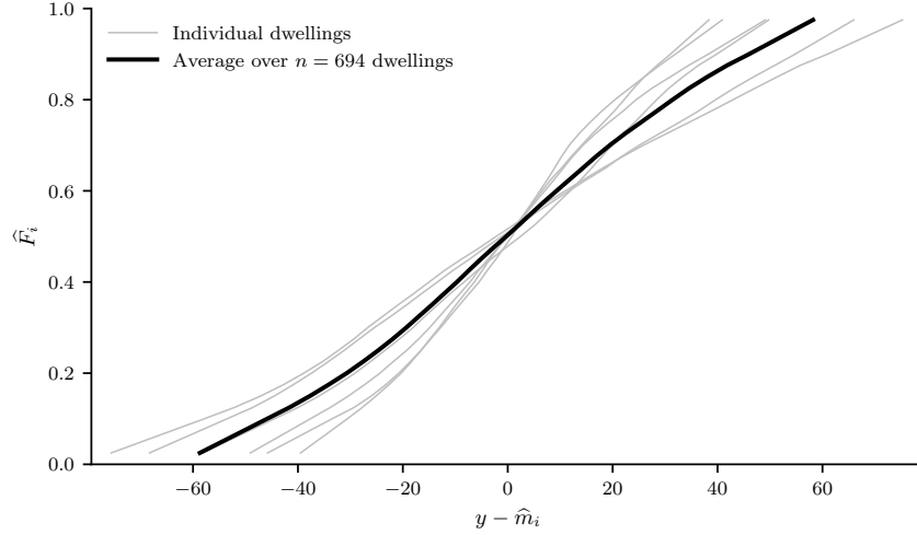
Figure 3: Example of distribution functions
