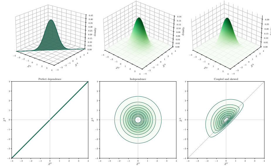
Figure 2: Copula dependence structures
