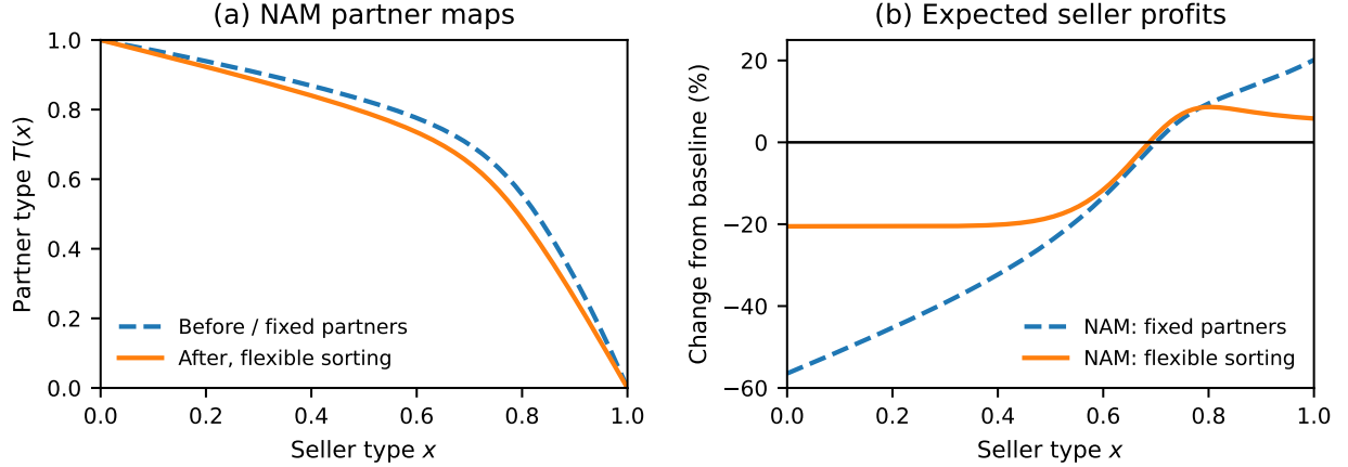
Figure 2: High-type supply reduction (Table 1, Panel A). Left: the baseline partner map, retained with fixed partners, and the new flexible assignment. Right: changes in expected profit per seller relative to baseline; the zero line marks unchanged profits. Both panels hold seller type x fixed. The right panel excludes changes in seller numbers.
