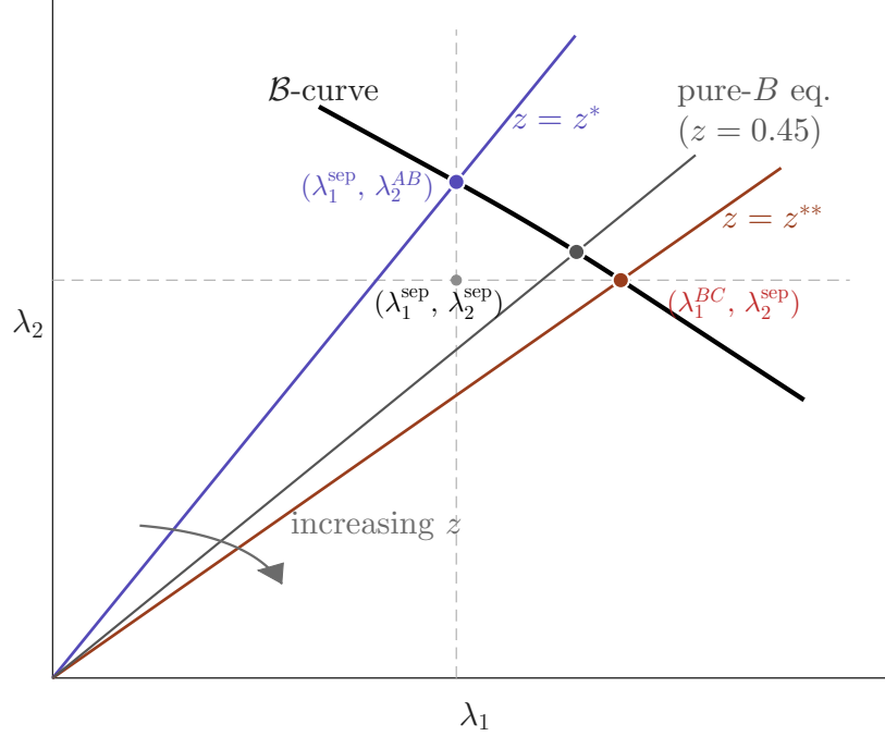
Figure 1: The \mathcal{B} -curve is the locus of queue-length pairs (\lambda_1, \lambda_2) consistent with seller optimality and buyer free entry when \alpha_B > 0 . The dashed lines mark the queue floors \lambda_1^{\text{sep}} , and the feasible portion of the curve is the segment between the blue AB point (\lambda_1^{\text{sep}}, \lambda_2^{\text{AB}}) and the red BC point (\lambda_1^{\text{BC}}, \lambda_2^{\text{sep}}) . Each ray from the origin corresponds to a seller composition z , with slope (1 - z)/z . Rays intersecting the interior support pure-B equilibria, while the endpoint rays define z^* and z^{**} . As z increases, the ray rotates clockwise. Parameters: x_{11} = 1 , x_{22} = 2 , x_{12} = 1.9 , K = 0.2 , and m(\lambda) = 1 - e^{-\lambda} , yielding \bar{x}_{12} = 1.435 , \lambda_1^{\text{sep}} = 0.88 , \lambda_2^{\text{sep}} = 1.31 , \lambda_2^{\text{AB}} = 1.63 , \lambda_1^{\text{BC}} = 1.24 , z^* = 0.35 , and z^{**} = 0.49 .
