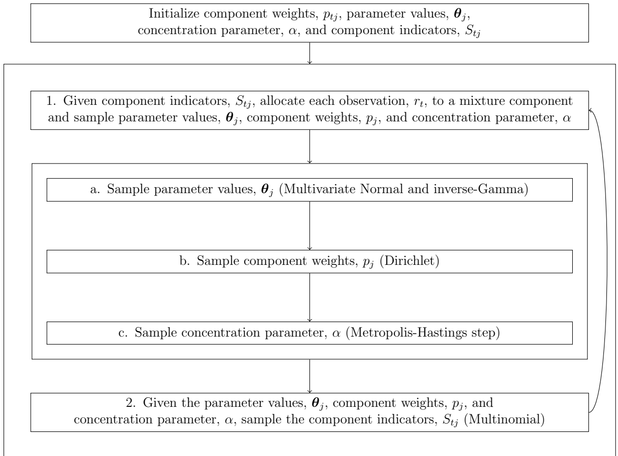
Figure A.1: Summary of the algorithm for the Sparse Finite Mixture Markov Chain Monte Carlo (SFM-MCMC) sampling procedure
