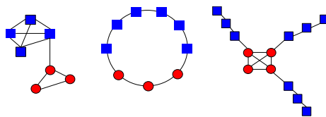
Stylized networks: Bridge (left), Ring (middle). Core-Periphery (right). Rich countries are represented by red circles and poor countries are represented by blue squares.
