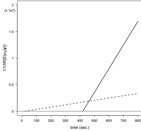
Figure 4: Precision of the importance sampling estimator of posterior mean for parameter \omega_2 , i.e., 1/\text{VAR}[E(\omega_2 | \mathbf{y})] , for the four-component mixture candidate (in solid line) and for the t_1 candidate (in dotted line).
