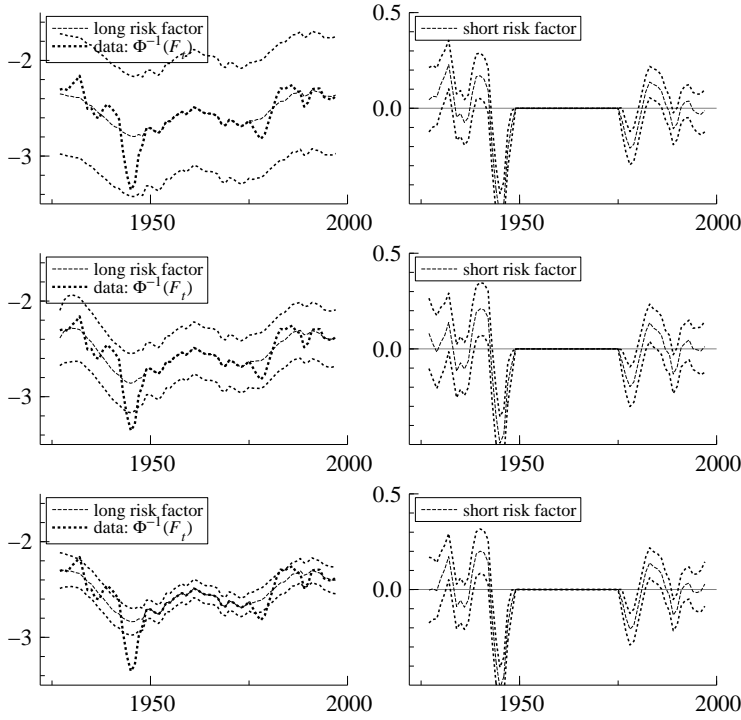
Figure 2: Dynamic Model Fit
