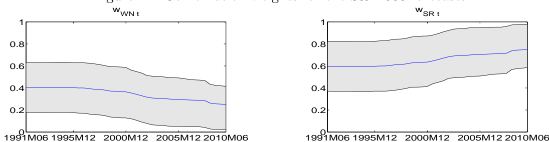
Figure 12: Combination weights for the S&P 500 forecasts
