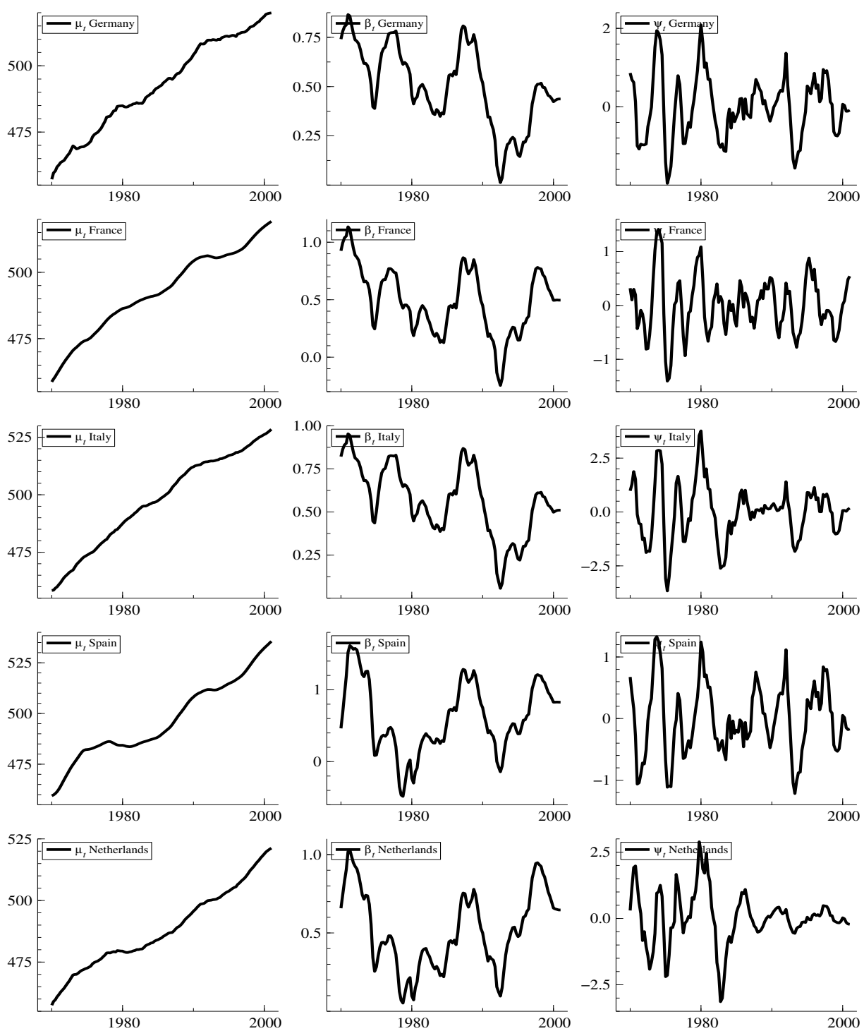
Figure 5: Trend, slope and cycle components for converging trend-cycle model.
